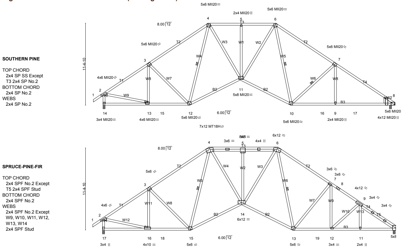
Figure 12 Roof Truss T1 – Flat (See Figure 10)
