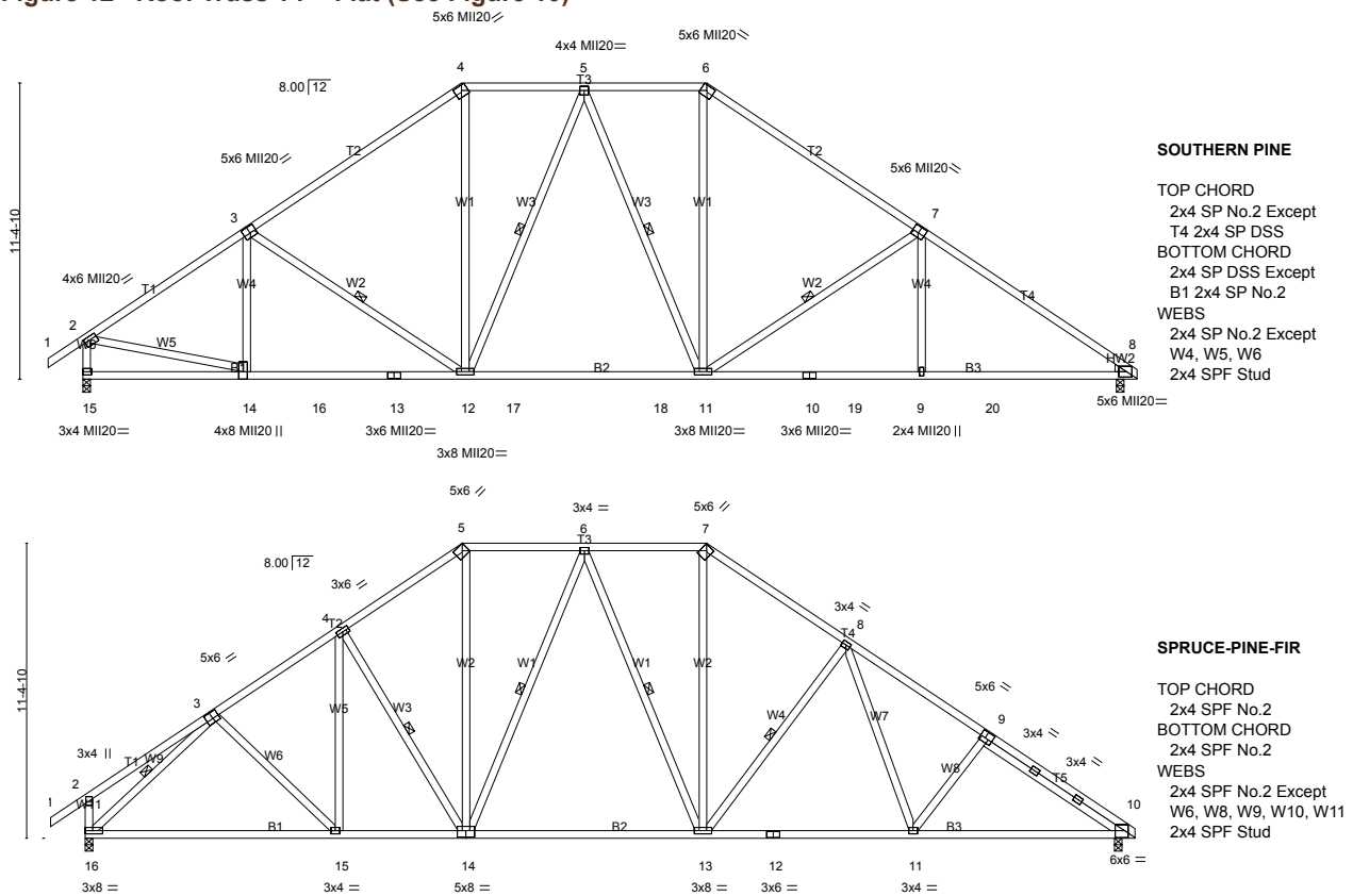
Figure 12 Roof Truss T1 – Flat (See Figure 10)
